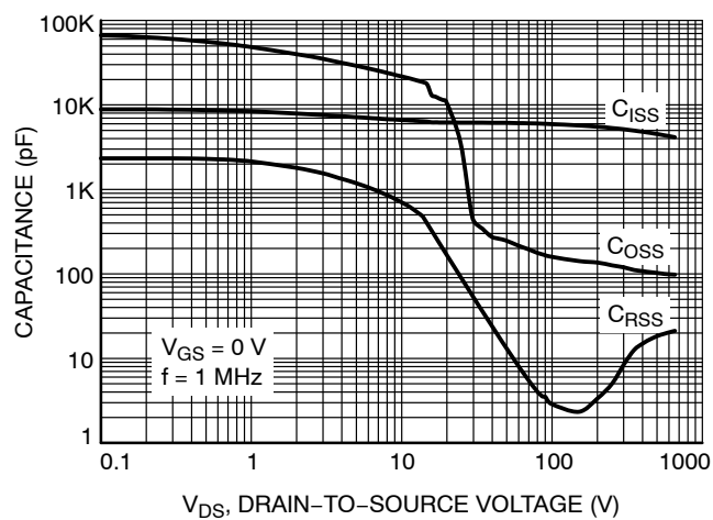
Figure 15. Capacitance Variation
