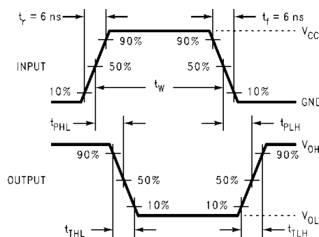
Figure 6. AC Waveforms
