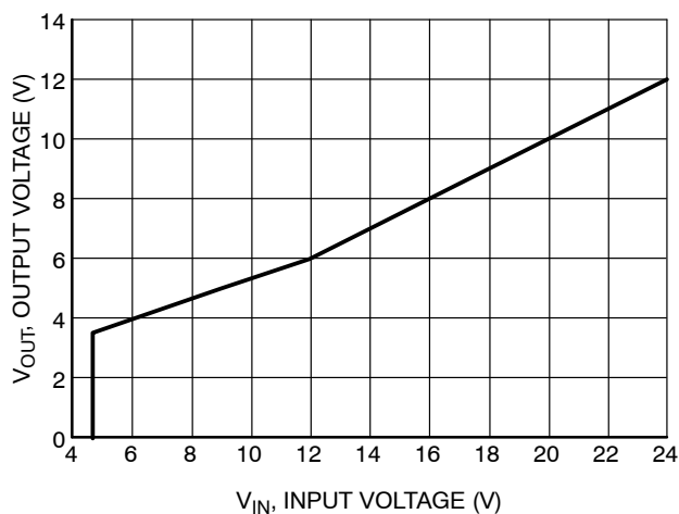
Figure 44. Recommended Maximum Output Voltage vs Input Voltage
