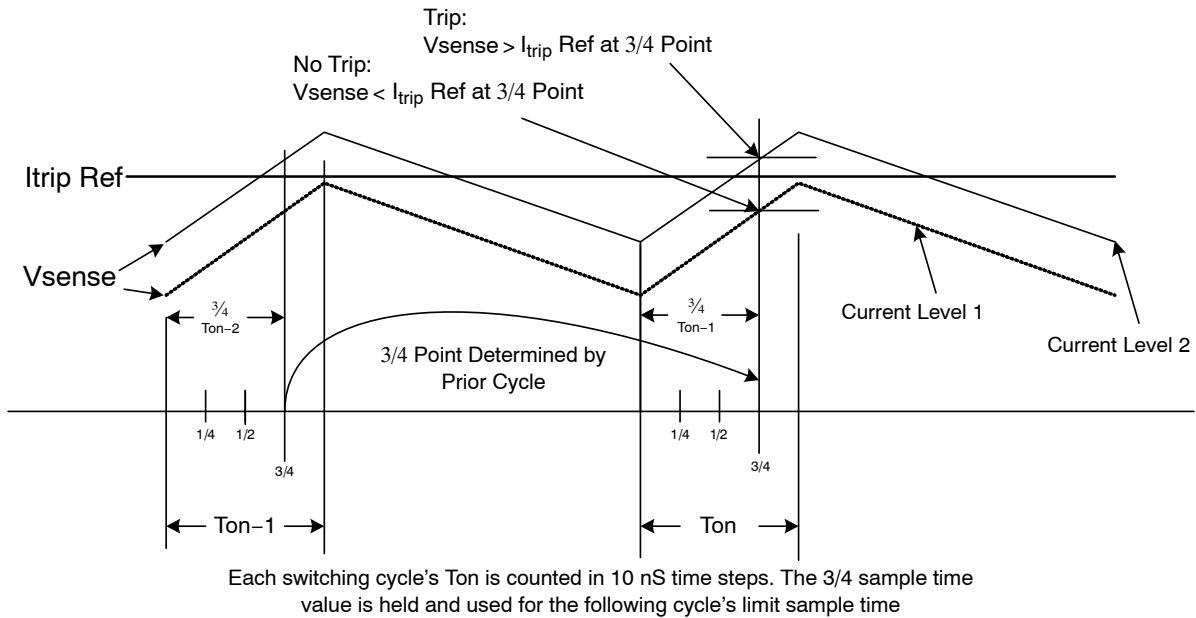
Figure 36. I_{Limit} Trip Point Description
