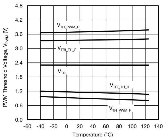
Fig. 16 - PWM Threshold vs. Temperature (SiC788)
